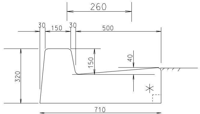
Barrier kerb and gutter adjacent to footway
