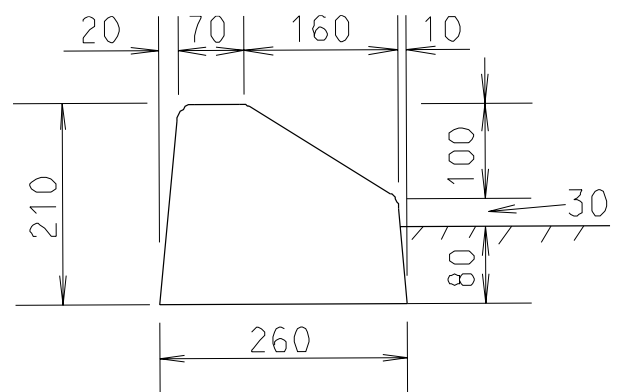
Raised median stripes and traffic islands
