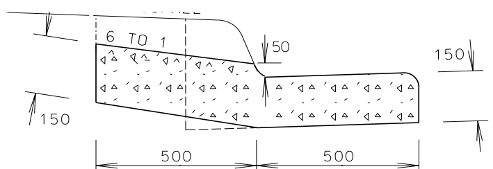
Footway crossfall
